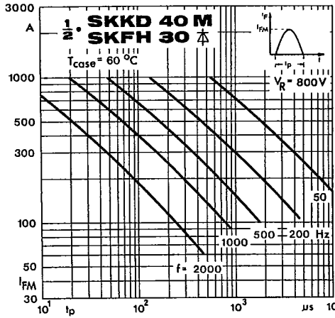
Fig. 12 d Rated sinusoidal peak forward current
