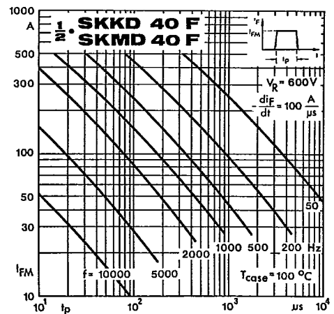
Fig. 14 c Rated rectangular peak forward current
