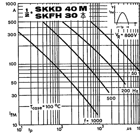
Fig. 12 f Rated sinusoidal peak forward current
