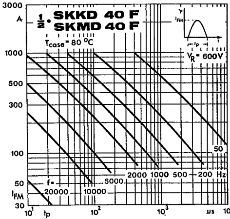
Fig. 12 b Rated sinusoidal peak forward current
