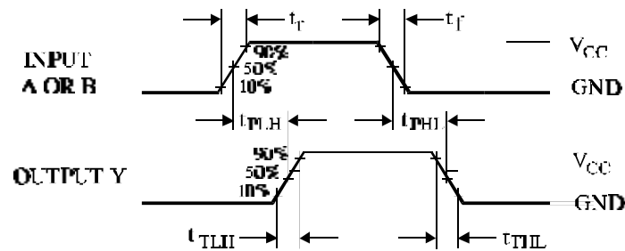
Figure 1. Switching Waveforms
