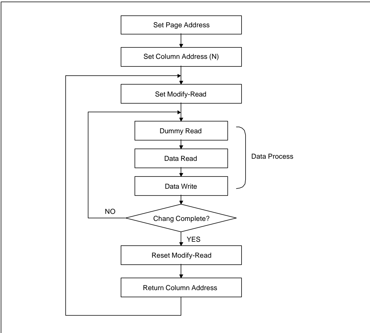
Figure 14. Sequence for Cursor Display
