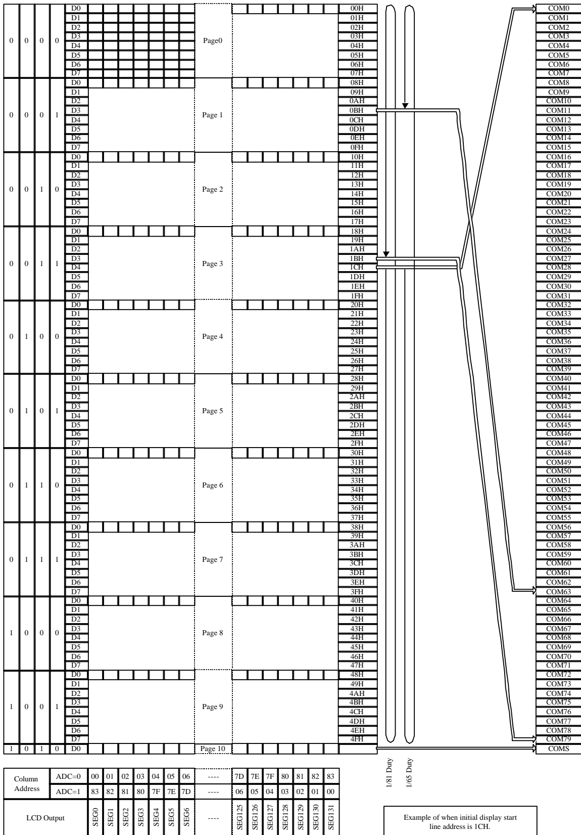
Figure 8. Display Data RAM Map (1/81, 1/65 duty mode)
