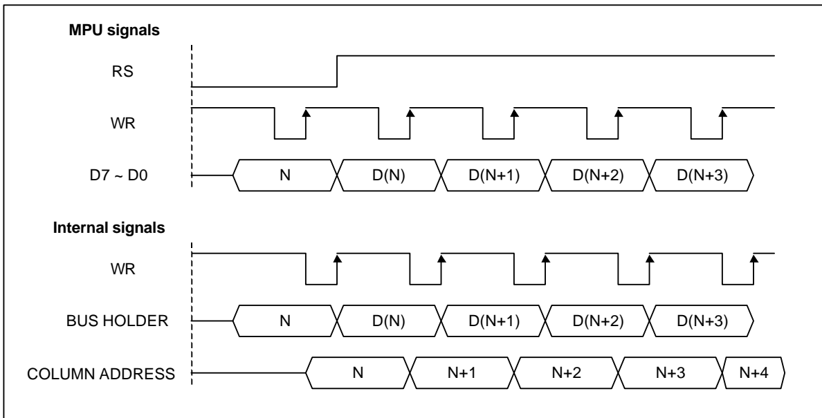
Figure 4. Write Timing
