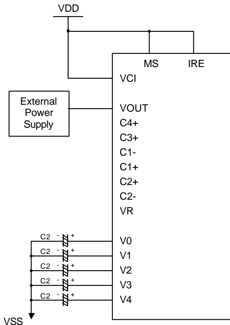
(c) Using internal voltage regulator resistors (IRE=1)
