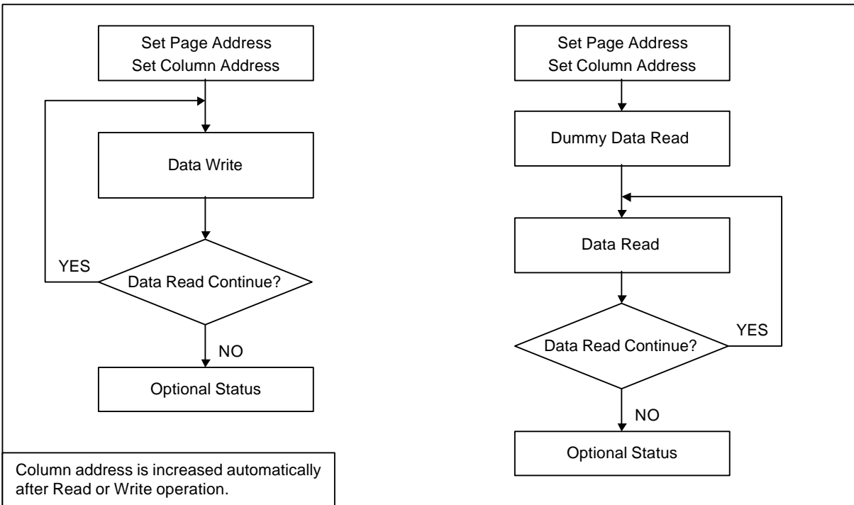
Figure 12. Sequence for Writing Display Data
