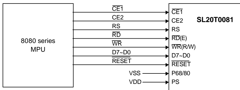
(b) 8080 Bus type interface
