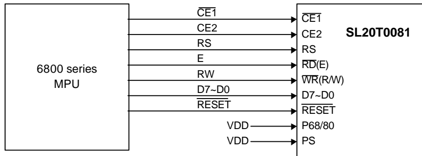
(a) 6800 Bus type interface
