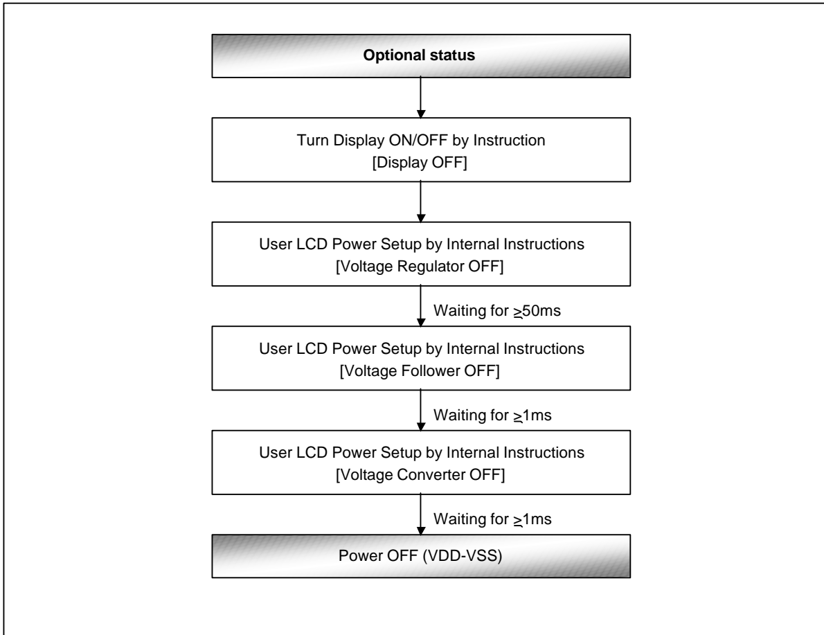
Figure 20. Power OFF
