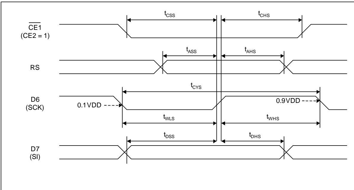
Figure 24. Serial Interface Characteristics
