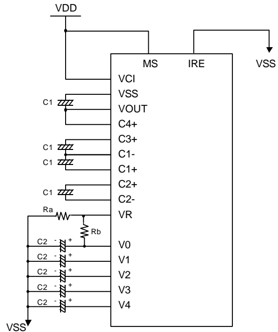
(b) Using external voltage regulator resistors (IRE=0)
