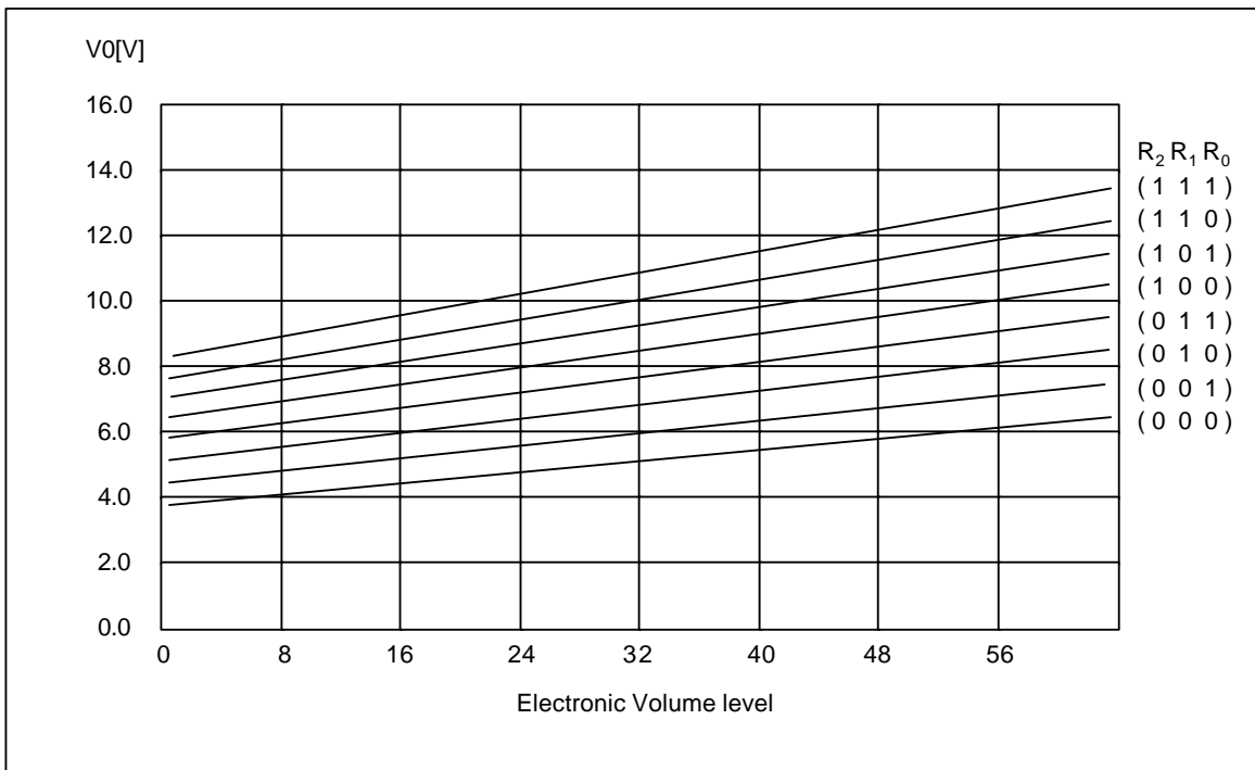
Figure 11. Electronic Volume Level
