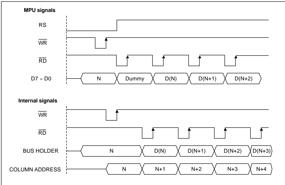
Figure 5. Read Timing
