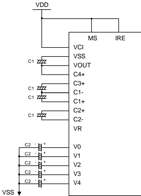
(a) Using internal voltage regulator resistors (IRE=1)
