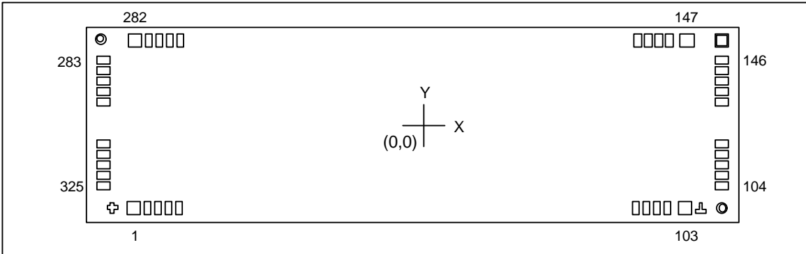
Figure 1. SL20T0081 PAD Layout
