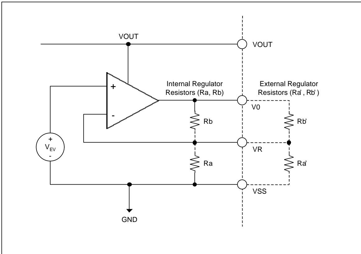
Figure 10. Internal Voltage Regulator Circuit
