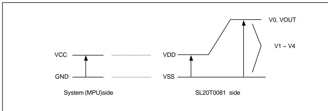
Figure 21. Relations between powers and V voltages
