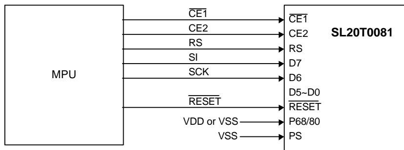
(c) Serial interface
