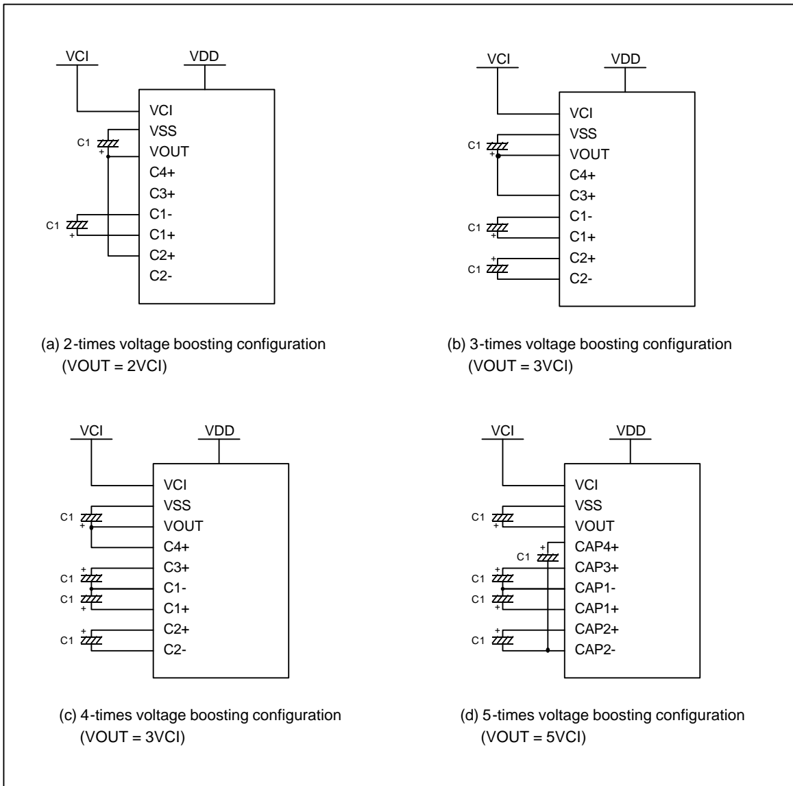
Figure 9. Power supply circuits for various voltage boosting
