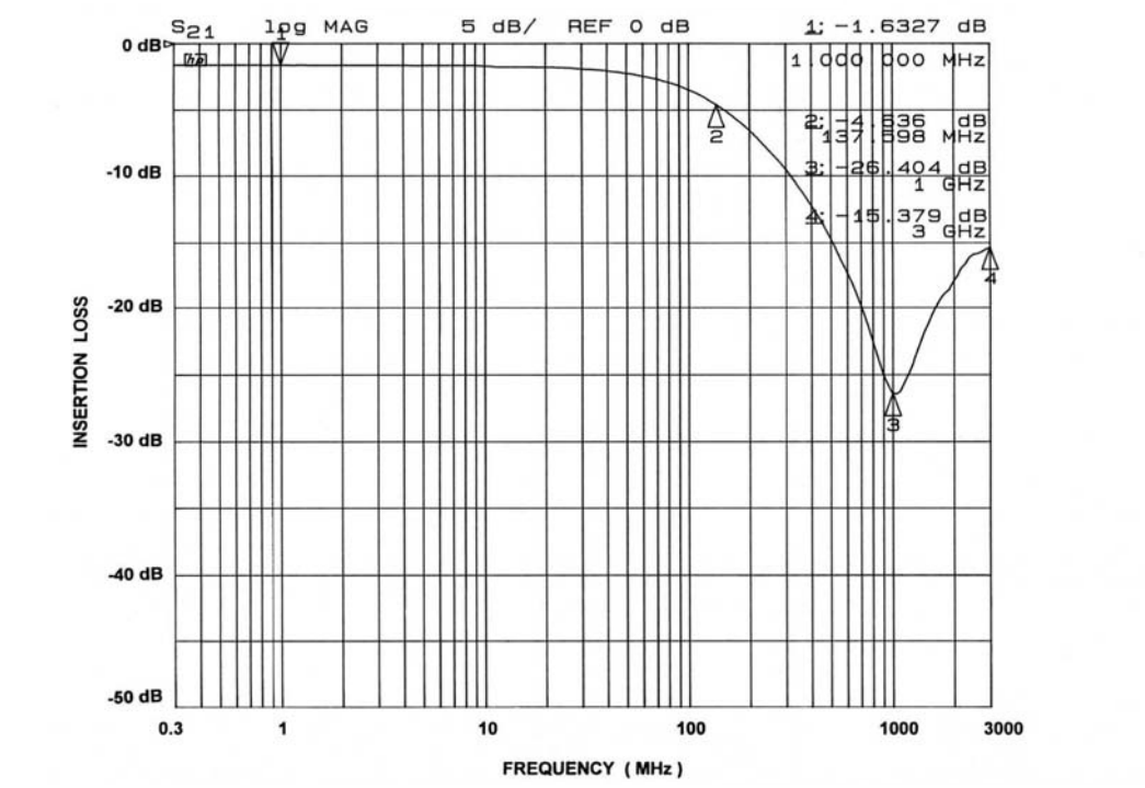
Figure 4. Insertion Loss vs. Frequency Performance Curve, PACUSB-D3(SOT23-6)
