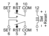
Reset condition
