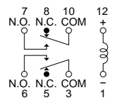
Deenergized condition
