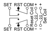
Reset condition
