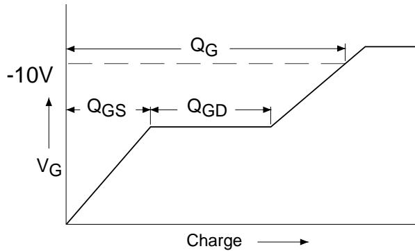
Fig 9a. Basic Gate Charge Waveform
