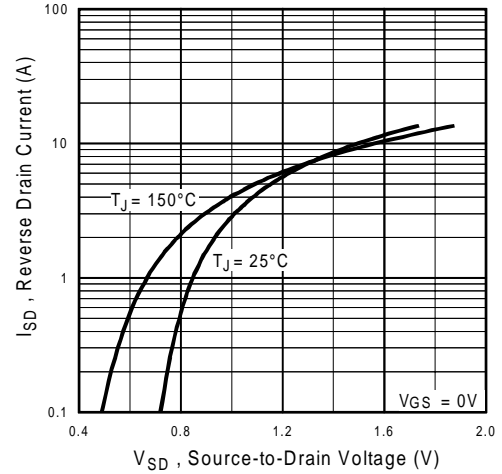
Fig 4. Typical Source-Drain Diode Forward Voltage
