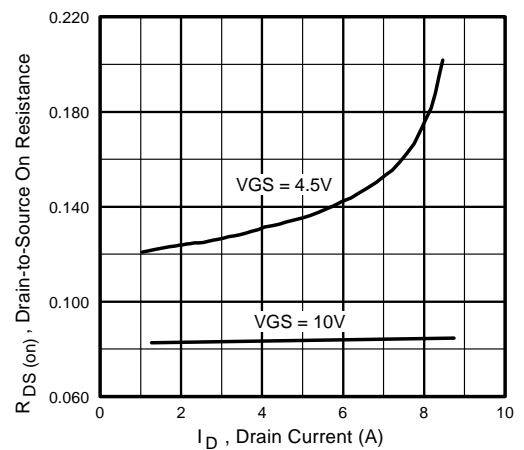
Fig 6. Typical On-Resistance Vs. Drain Current
