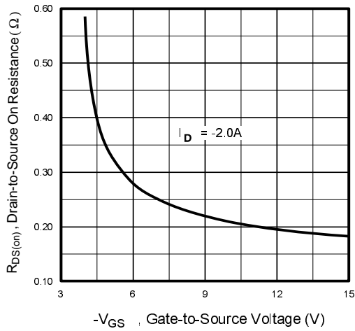
Fig 17. Typical On-Resistance Vs. Gate Voltage
