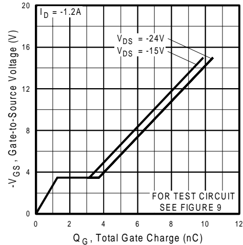
Fig 20. Typical Gate Charge Vs. Gate-to-Source Voltage
