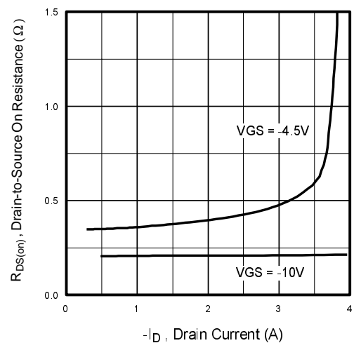
Fig 16. Typical On-Resistance Vs. Drain Current
