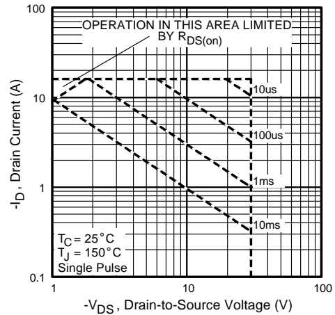
Fig 18. Maximum Safe Operating Area
