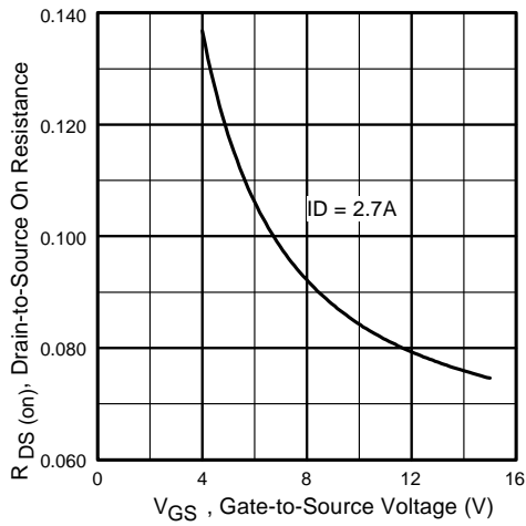
Fig 7. Typical On-Resistance Vs. Gate Voltage
