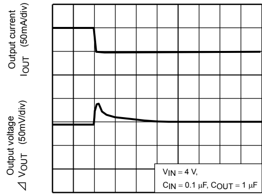
TCR5SB30 ( I_{OUT} = 100m to 50mA )
