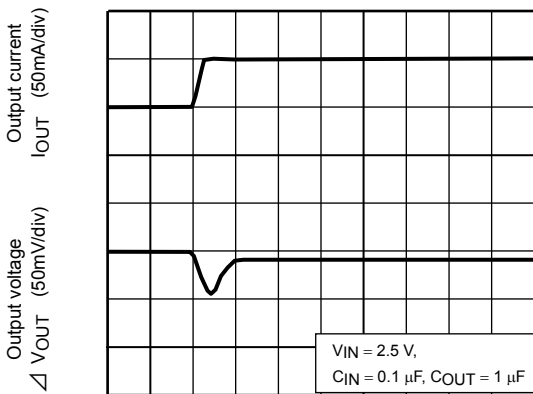
TCR5SB15 ( I_{OUT} = 50m to 100mA )
