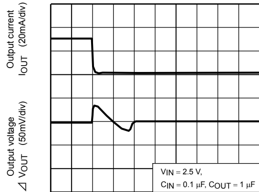
TCR5SB15 ( I_{OUT} = 30m to 1mA )
