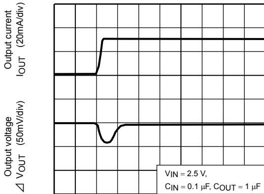
TCR5SB15 ( I_{OUT} = 1m to 30mA )
