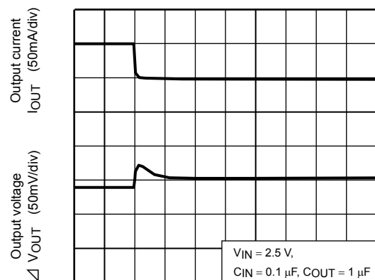
TCR5SB15 ( I_{OUT} = 100m to 50mA )
