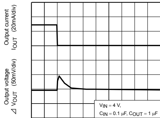
TCR5SB30 ( I_{OUT} = 30m to 1mA )
