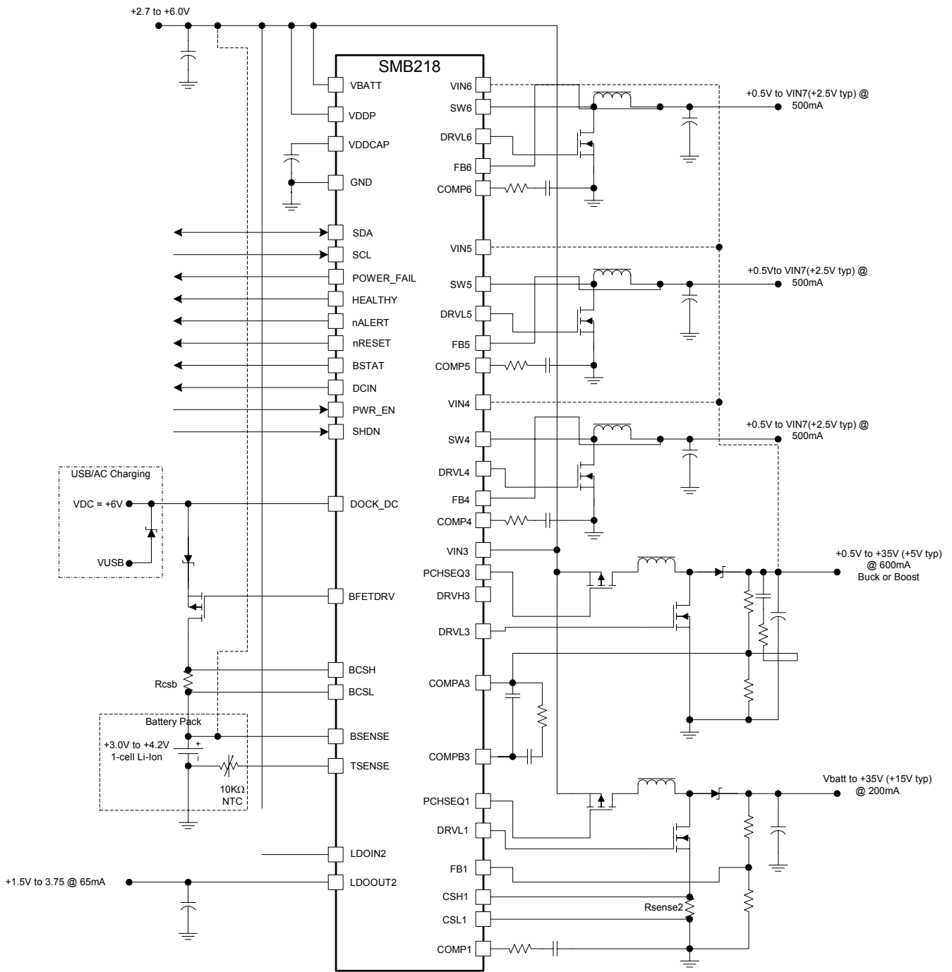
Figure 2a – Typical application schematic of the SMB218 (QFN-48) showing external circuitry necessary to configure the output channels as: step-up, LDO, step-down outputs and battery charger.
