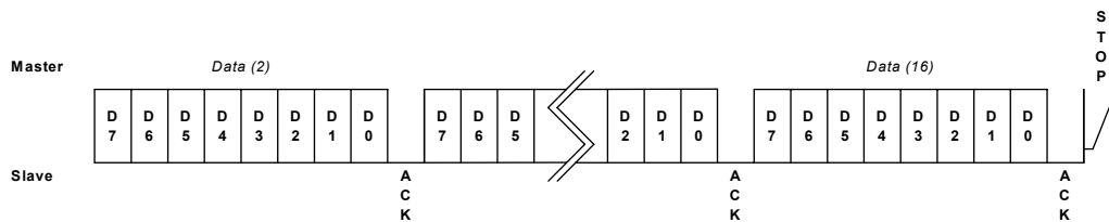
Figure 19 - General Purpose Memory Page Write
