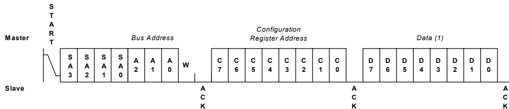
Figure 18- General Purpose Memory Byte Write
