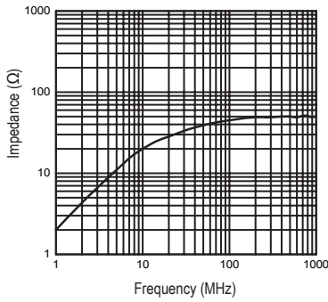
Typical Z vs Frequency
