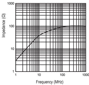
Typical Z vs Frequency
