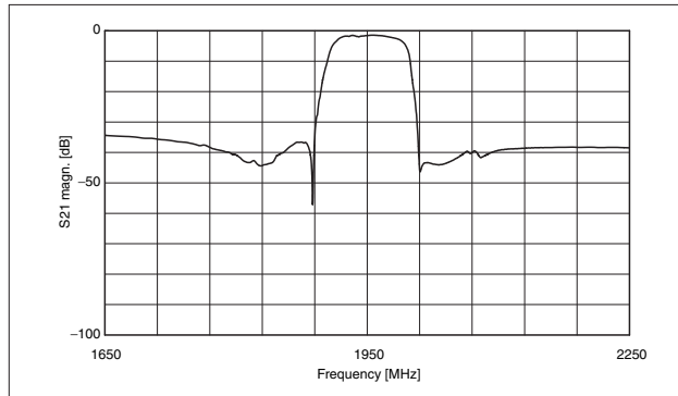
<W-CDMA Tx> Parts No.: SF14-1950M5UU00
