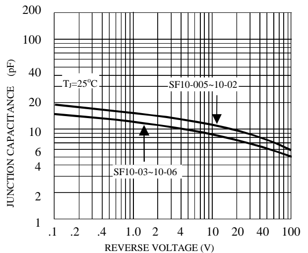
FIG. 6-TYPICAL JUNCTION CAPACITANCE
