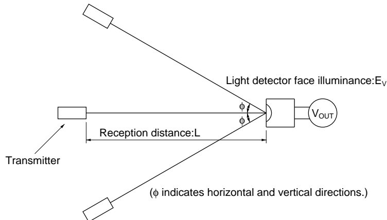
Fig.2 Standard Optical System
