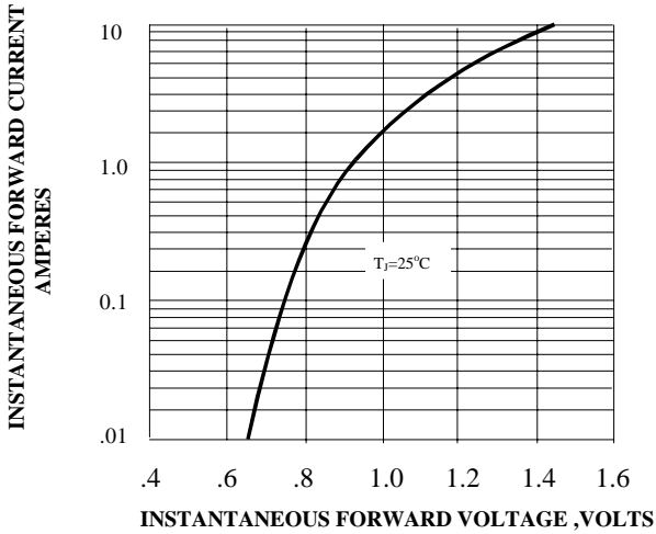
FIG. 3-TYPICAL FORWARD CHARACTERISTICS
