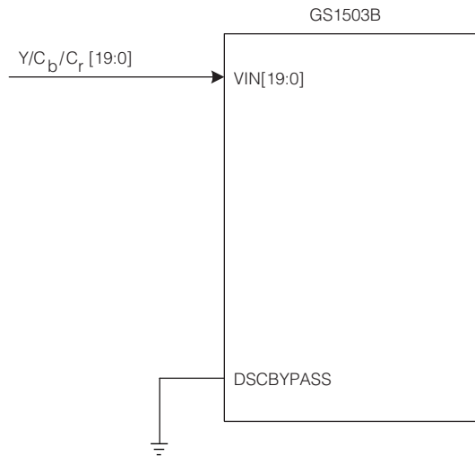
Figure 5-1: 20-bit Scrambled Input Configuration
