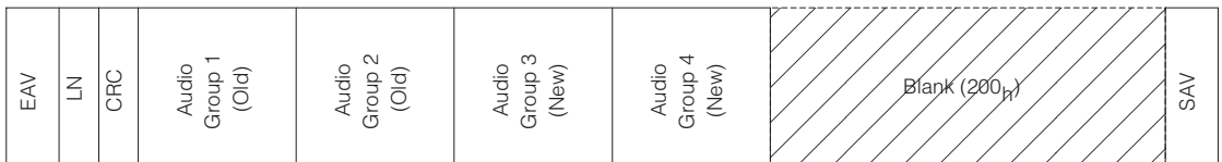
Video Signal after GS1503B Insertion of Audio Groups 3 & 4 (CASCADE = 1)
