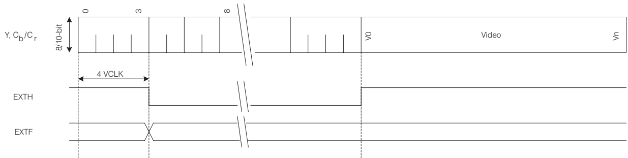
Figure 4-6: Video Input Format (8/10-bit without TRS and Line Numbers)
