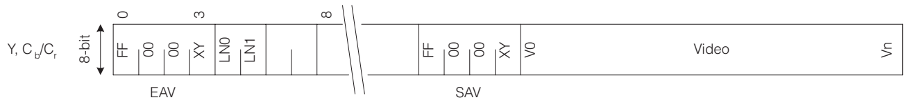
Figure 4-4: Video Input Format 8-bit with TRS and Line Numbers
