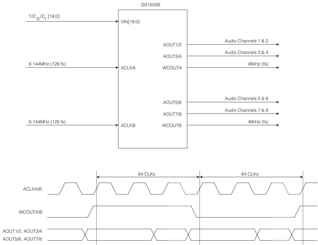
Figure 5-8: Serial Audio Output Configuration and Timing
