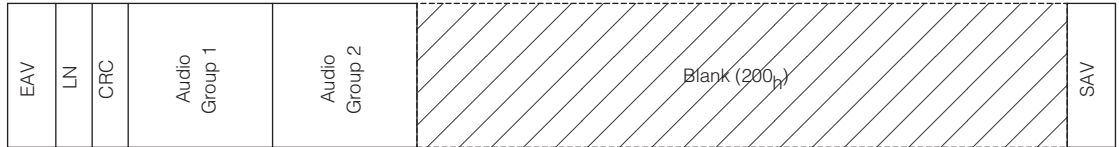
Video Signal before GS1503B (with existing Audio Data Packets)
