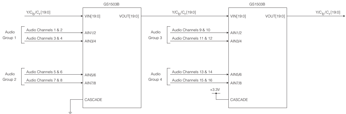
Figure 4-16: Multiplexing 16 Channels of Audio using Cascade Architecture
