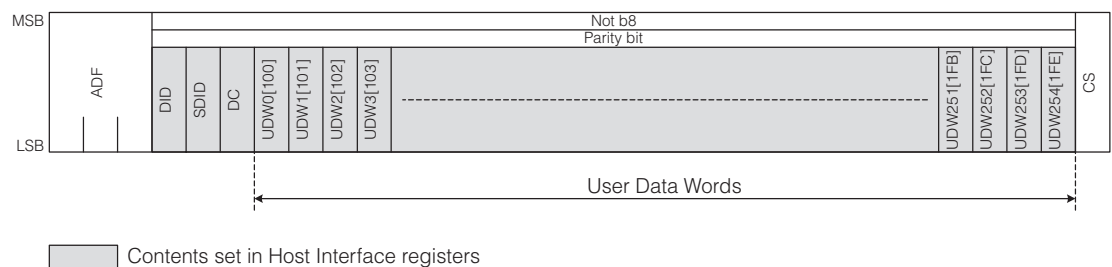
Figure 4-21: Arbitrary Data Packet Structure
