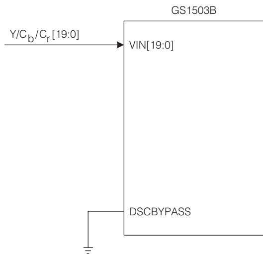
Figure 4-8: Configuration for 20-bit Scrambled Input
