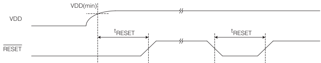
Figure 2-5: Reset Timing
