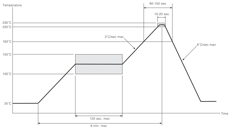
Figure 2-6: Maximum Pb-Free Solder Reflow Profile (Preferred)
