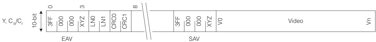
Figure 4-2: Video Input Format 10-bit with TRS and Line Numbers
