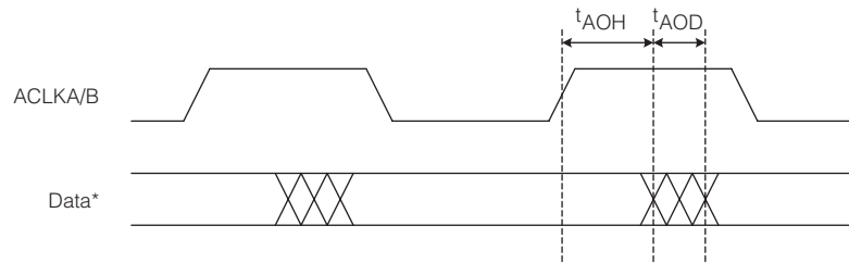
Figure 2-4: Audio Data Output Delay & Hold Time
