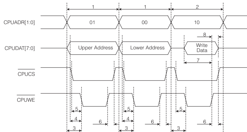
Figure 3-3: Host Interface Mode B Write Cycle Timing (CPU_SEL set LOW)
