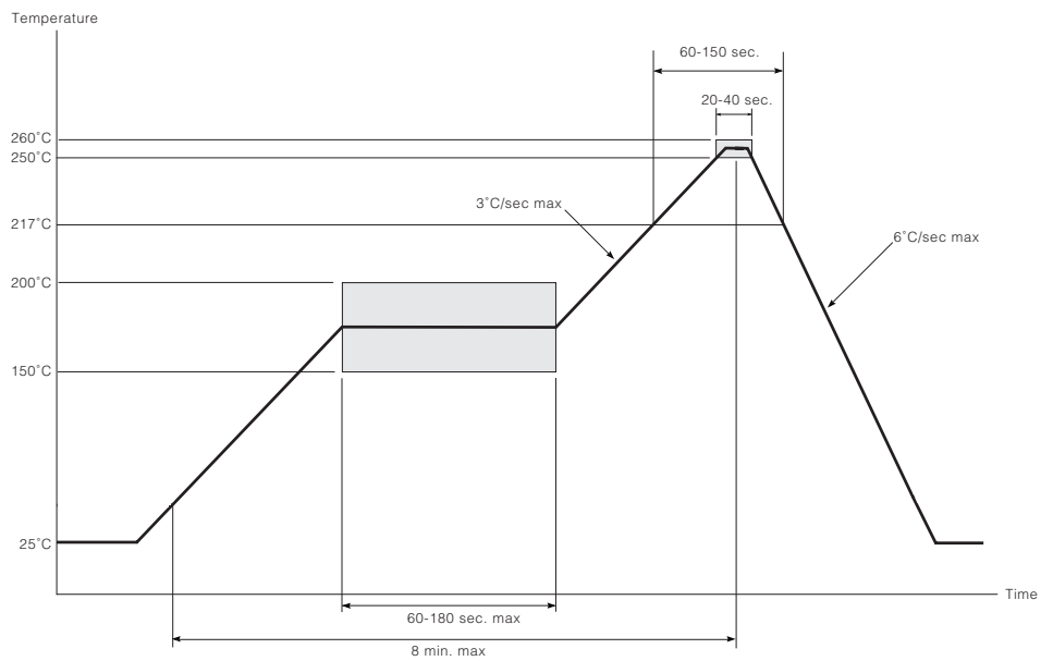
Figure 2-7: Standard Eutectic Solder Reflow Profile
