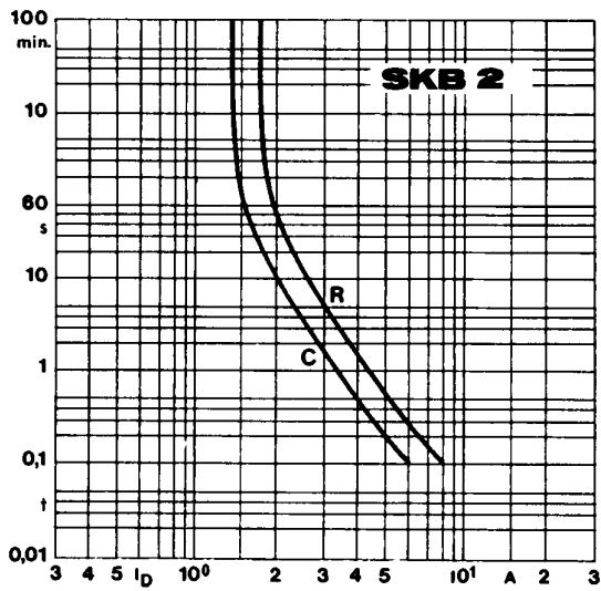
Fig. 6 Rated overload current vs. time
