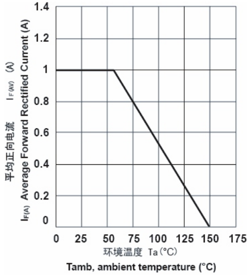
FIG. 1 – DERATING CURVE FOR OUTPUT RECTIFIER CURRENT
