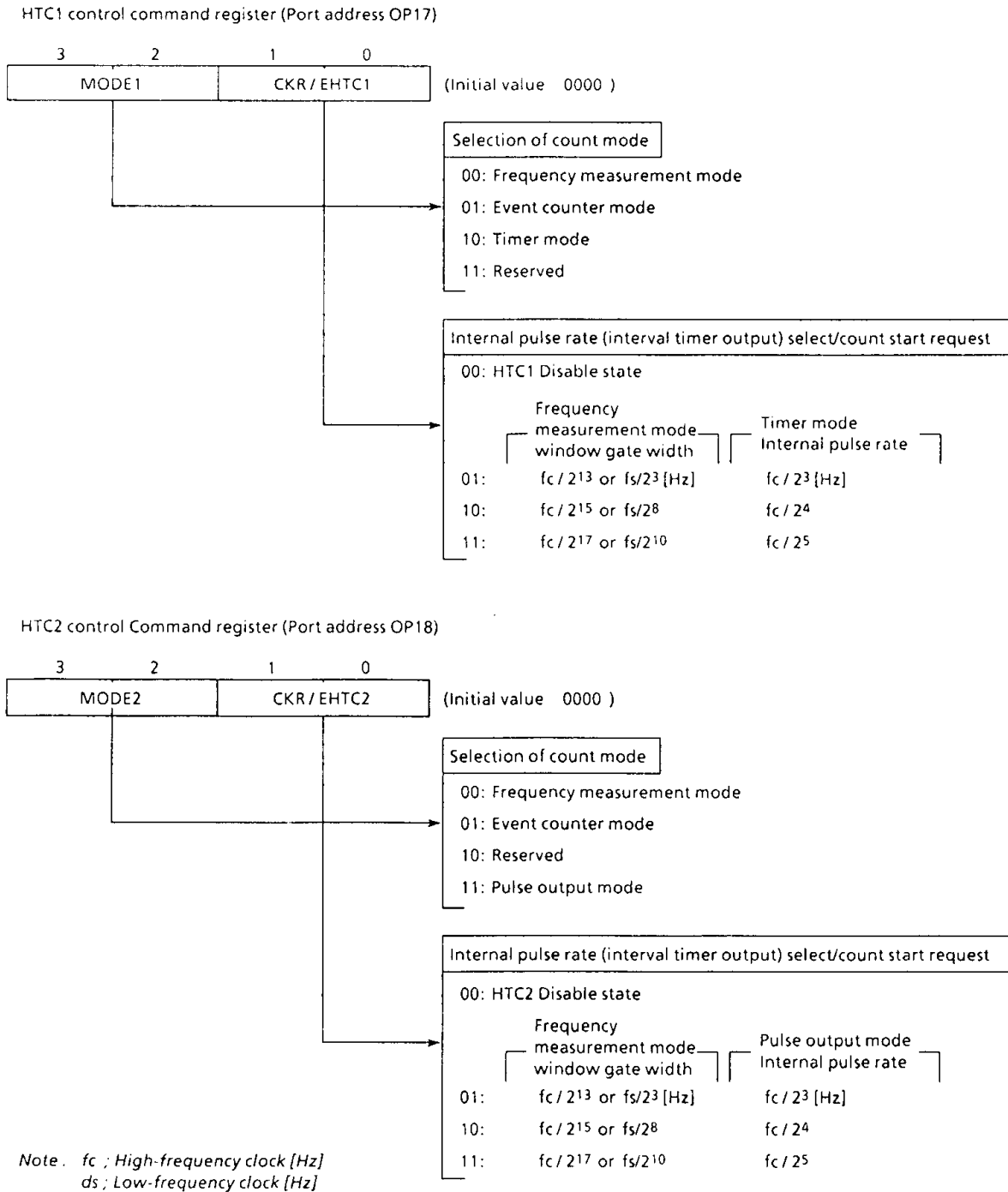
Figure 2-4. HTC1, HTC2 control Command register
