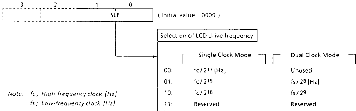
LCD Driver control command register 1 (Port address OP1A)
