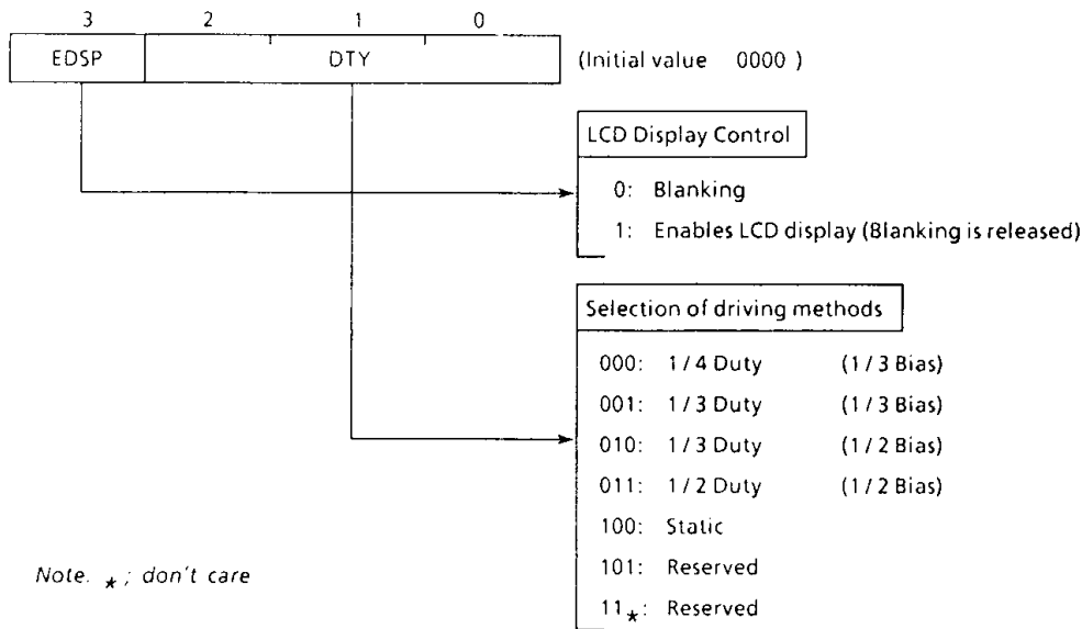
LCD Driver control command register 2 (Port address OP1B)
