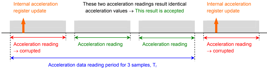
Figure 25. Interrupt based CMA3000 acceleration data read timing.
