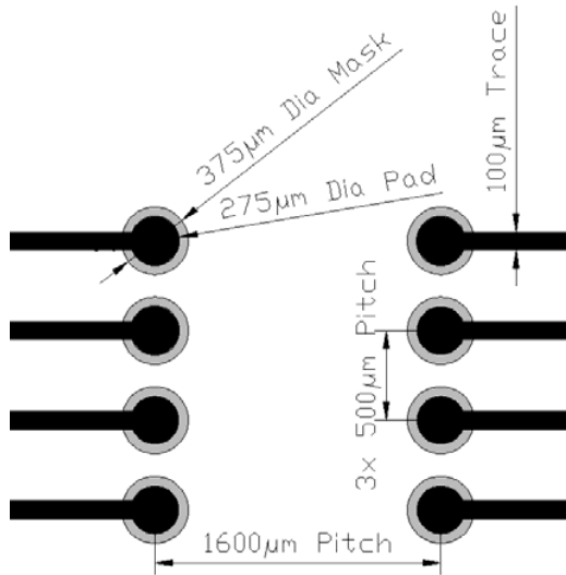
Figure 16. Recommended PWB pad layout for CMA3000.
