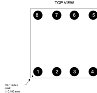
Figure 14. CMA3000 pin numbers
