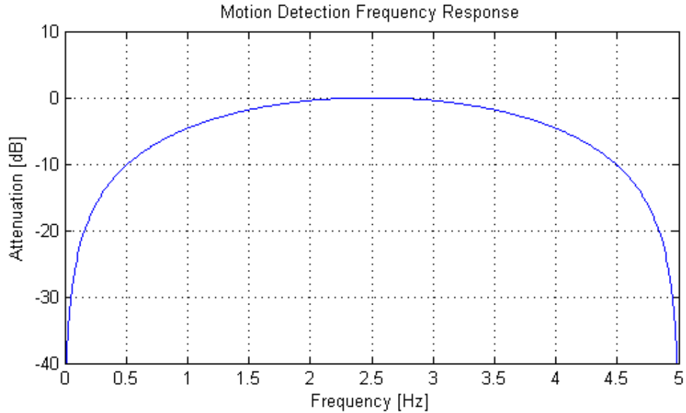
Figure 3. The MD band-pass filter's frequency response.
