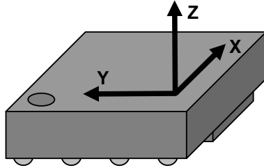
Figure 13. CMA3000 sensing directions
