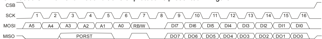
Figure 7. SPI frame format
