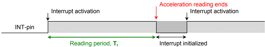
Figure 24. Interrupt based CMA3000 acceleration data read timing.
