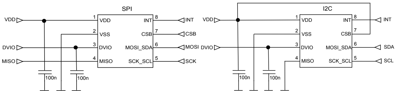
Figure 15 Recommended circuit diagrams for CMA3000-D0X
