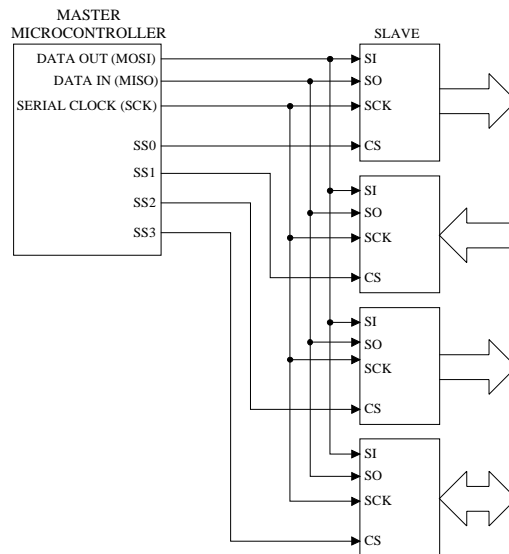
Figure 6. Typical SPI connection
