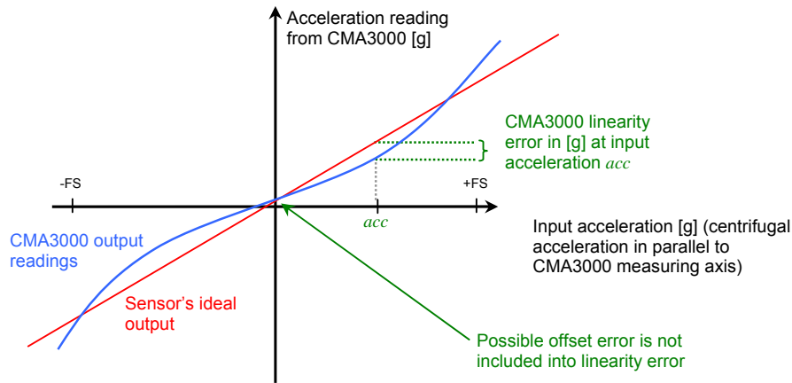
Figure 21. CMA3000's linearity error at input acceleration acc .
