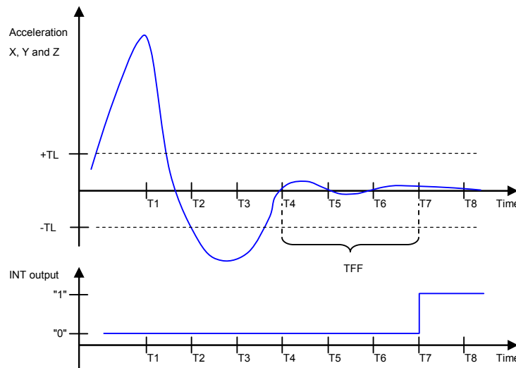
Figure 5. Free Fall condition
