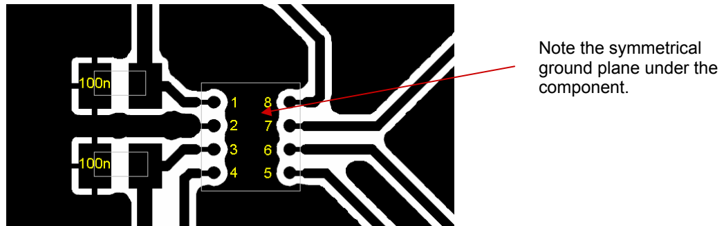
Figure 17. Recommended PWB layout for CMA3000-D0X with SPI interface (not actual size, for reference only).
