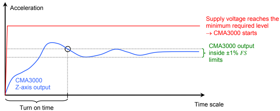
Figure 23. Turn-on time definition for one axis.
