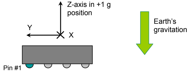
Figure 18. CMA3000 offset (0 g) position.
