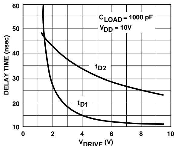
Effect of Input Amplitude on Delay Time
