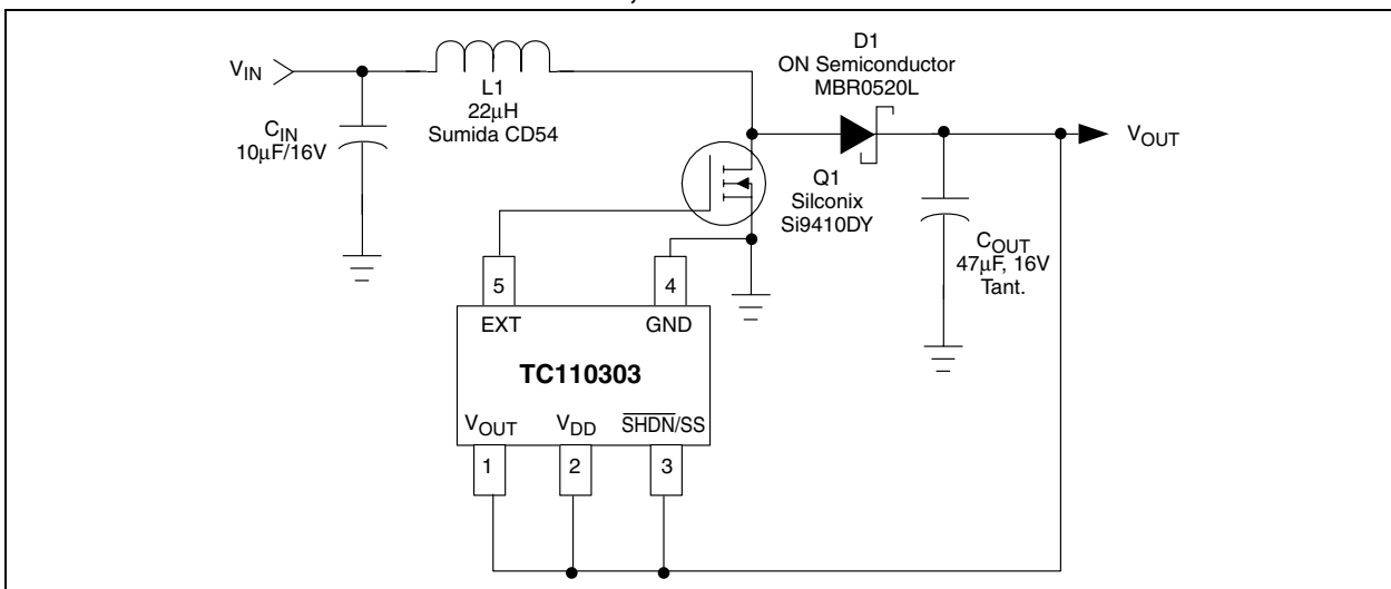
FIGURE 4-2: 300kHz BOOTSTRAPPED, N-CHANNEL TRANSISTOR
