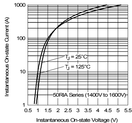
Fig. 14 - Forward Voltage Drop Characteristics
