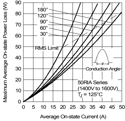
Fig. 9 - On-state Power Loss Characteristics
