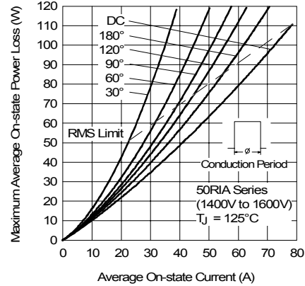
Fig. 10 - On-state Power Loss Characteristics
