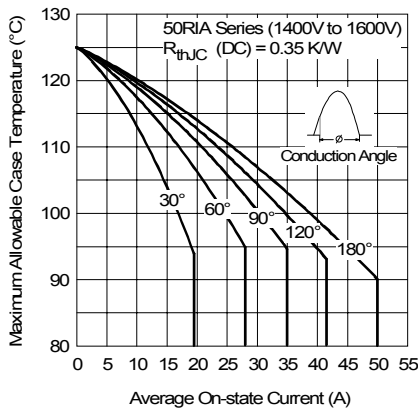
Fig. 7 - Current Ratings Characteristics
