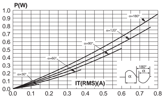
Fig 1: Maximum power dissipation versus RMS on-state current.
