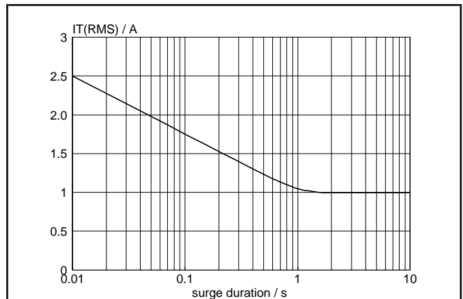
Fig.5. Maximum permissible repetitive rms on-state current I_{T(RMS)} , versus surge duration, for sinusoidal currents, f = 50\text{ Hz} ; T_{lead} \leq 108^\circ\text{C} .
