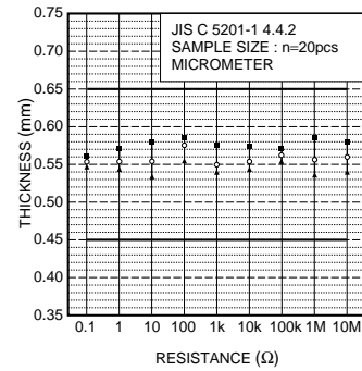
Fig.4 Dimensions (thickness)
