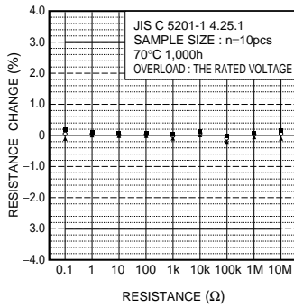
Fig.11 Endurance (at 70°C)
