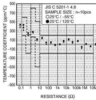
Fig.6 Variation resistance with temperature
