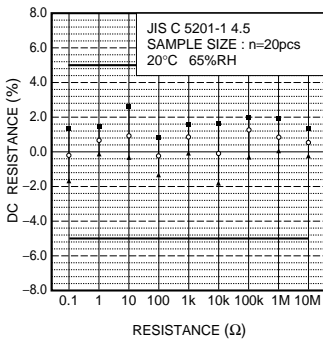
Fig.5 Resistance
