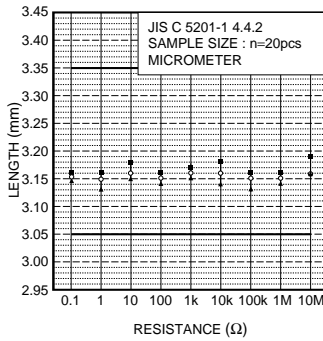
Fig.2 Dimensions (length)
