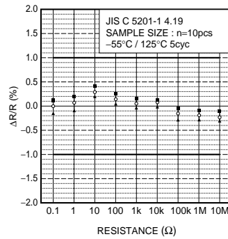
Fig.9 Rapid change of temperature
