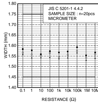
Fig.3 Dimensions (width)
