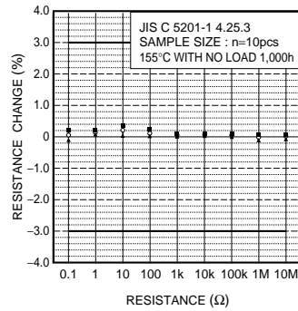
Fig.12 Endurance
