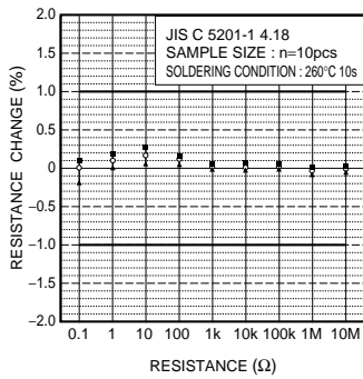
Fig.8 Resistance to soldering heat
