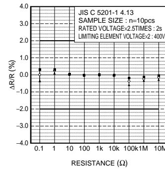
Fig.7 Overload
