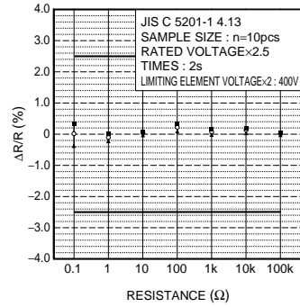
Fig.7 過負荷
