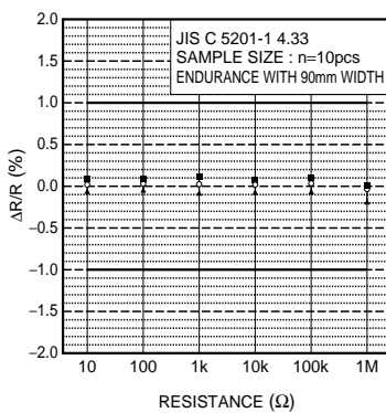
Fig.14 Bend strength of the end face plating
