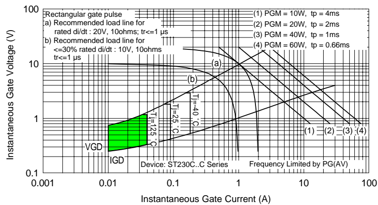
Fig. 11 - Gate Characteristics
