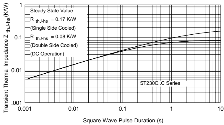
Fig. 10 - Thermal Impedance Z_{thJ-hs} Characteristics
