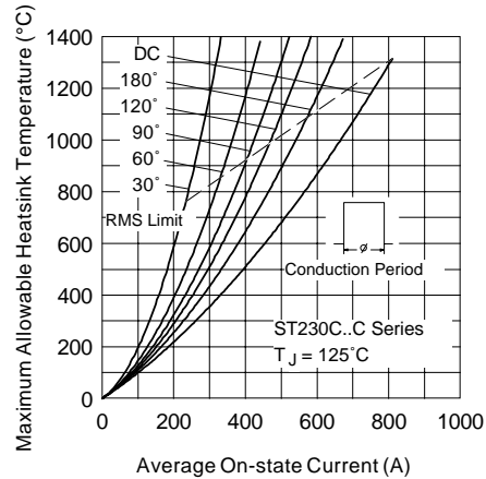
Fig. 6 - On-state Power Loss Characteristics
