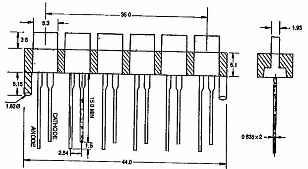
H-4 1.8x5.3m/m ARRAY SOCKET 6 SEGUENT
