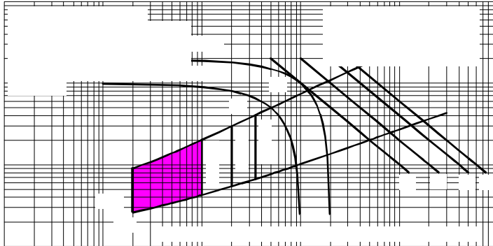
Fig. 17 - Gate Characteristics
