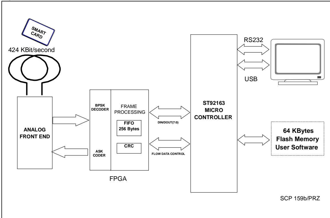
Figure 1 Contactless Reader Architecture with ST9
