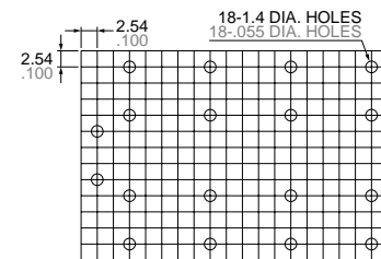
Tolerance: ±0.1 ±.004
