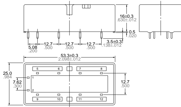
General tolerance: ±0.3 ±.012
