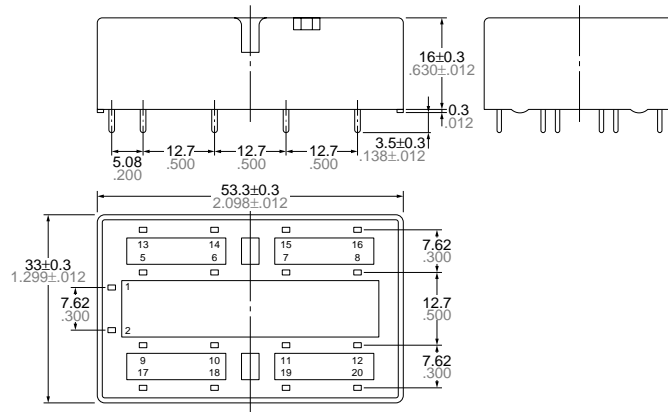
General tolerance: ±0.3 ±.012
