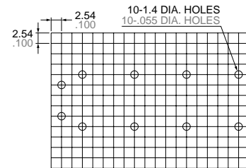
Tolerance: ±0.1 ±.004
