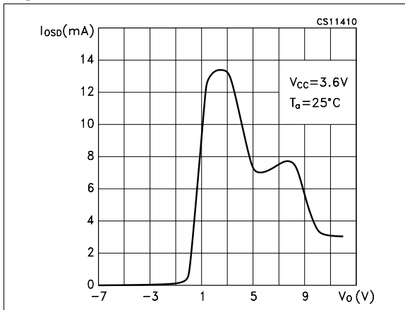
Figure 26. Driver short circuit current
