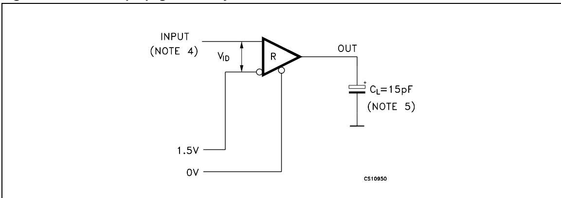
Figure 13. Receiver propagation delay time test circuit
