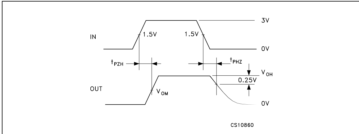
Figure 8. Drive enable and disable times waveforms
