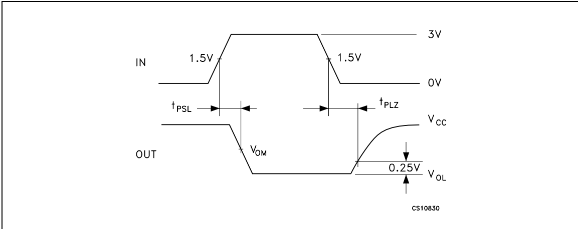
Figure 12. Drive enable and disable times waveforms
