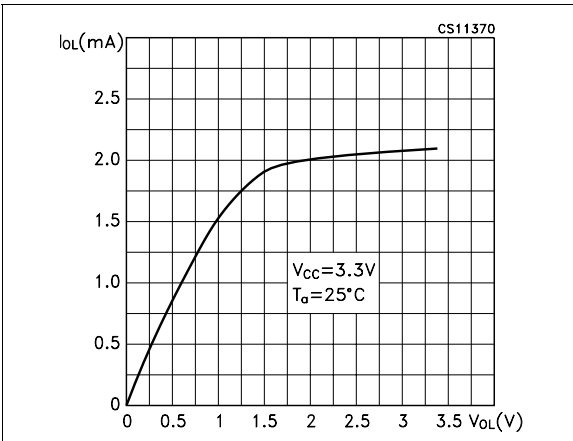
Figure 22. Low level driver output capability
