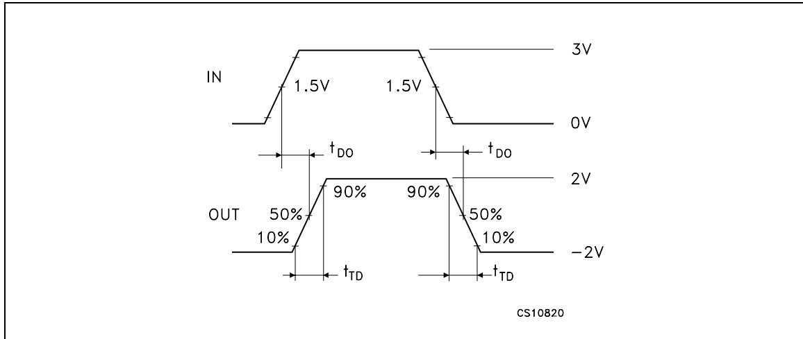
Figure 6. Drive differential output delay transition time waveform
