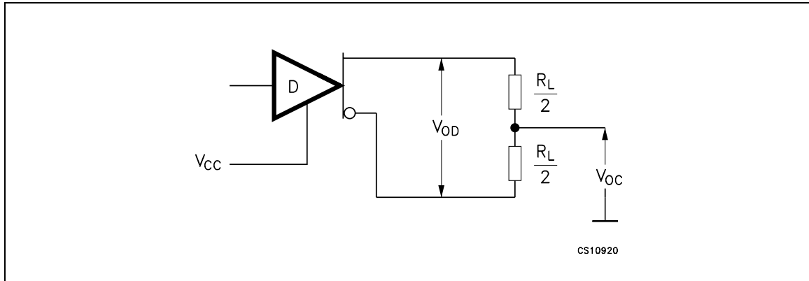
Figure 2. Driver and V_{OC} test load
