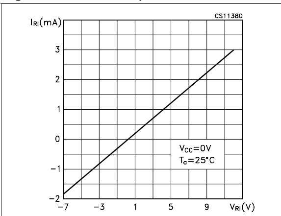
Figure 24. Receiver input characteristics
