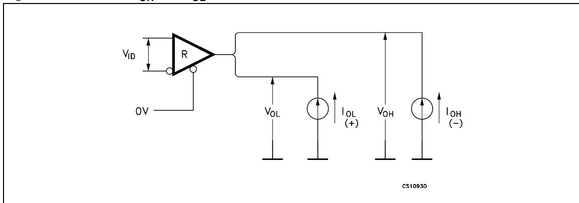
Figure 4. Receiver V_{OH} and V_{OL} test circuit
