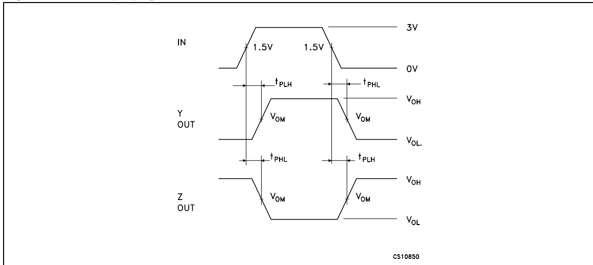
Figure 10. Drive propagation time waveform
