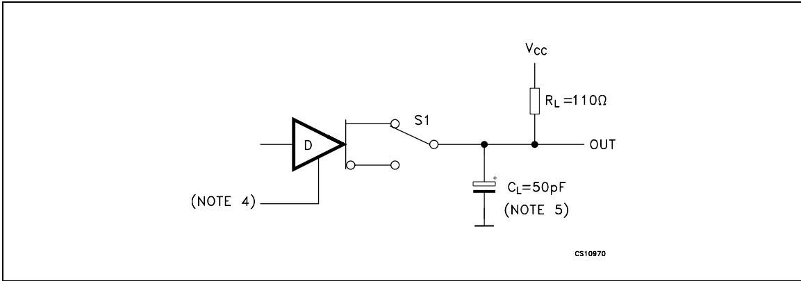
Figure 11. Drive enable and disable times test circuit
