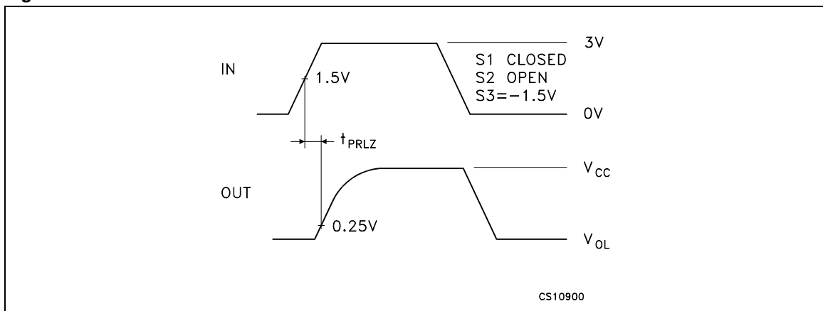
Figure 19. Receiver enable and disable times waveform
