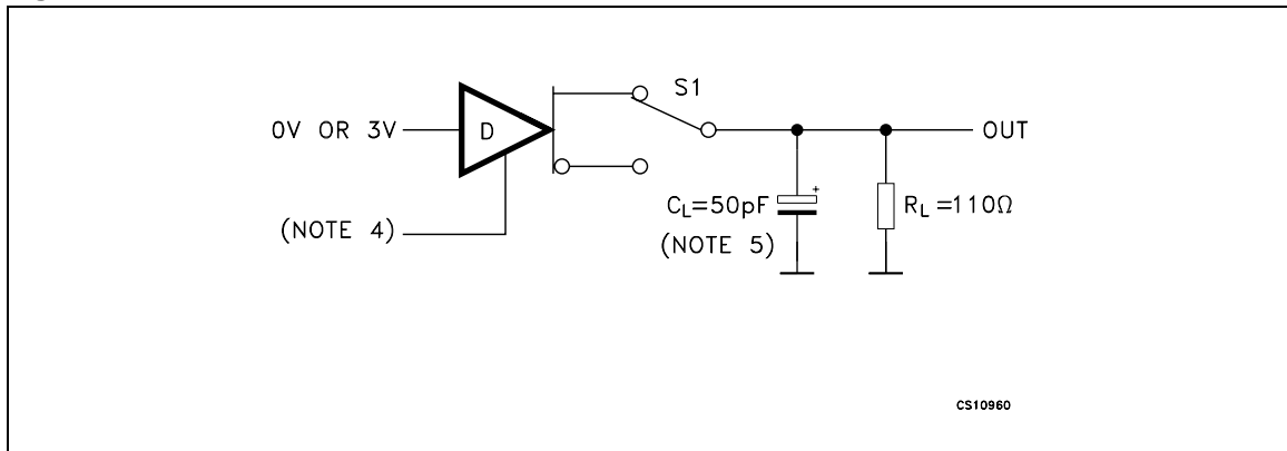
Figure 7. Drive enable and disable times test circuit
