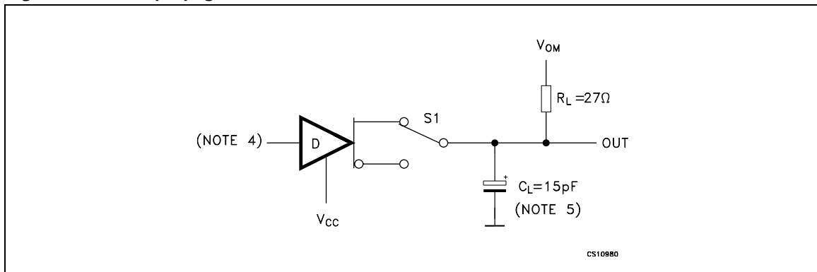
Figure 9. Drive propagation time test circuit
