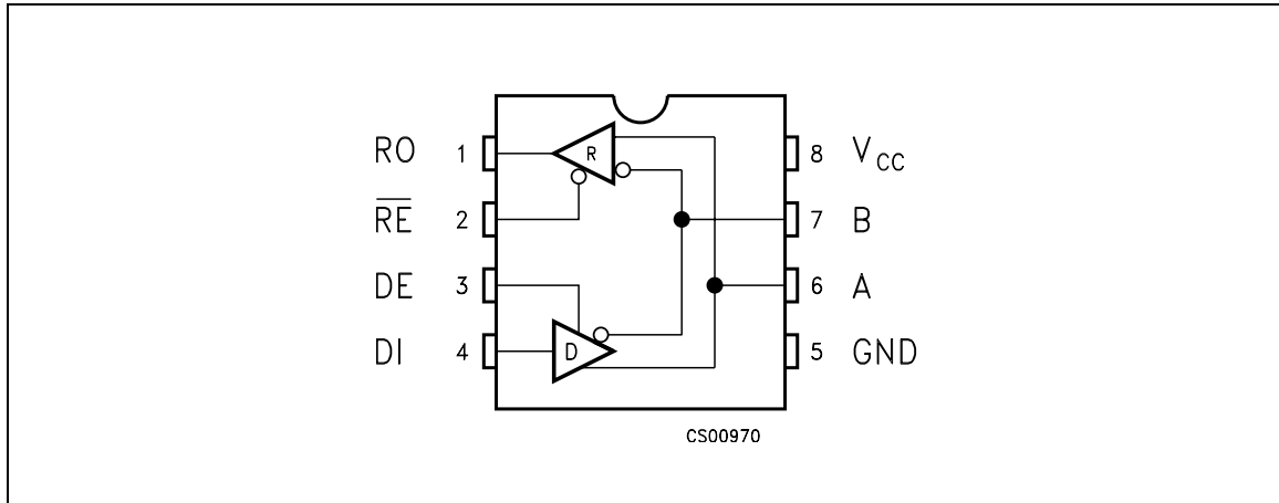
Figure 1. Pin connections
