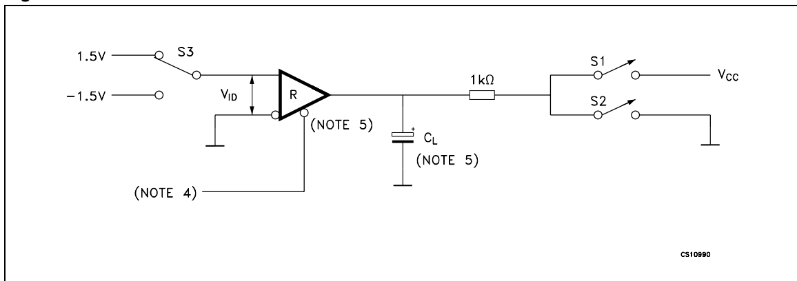
Figure 15. Receiver enable and disable times test circuit
