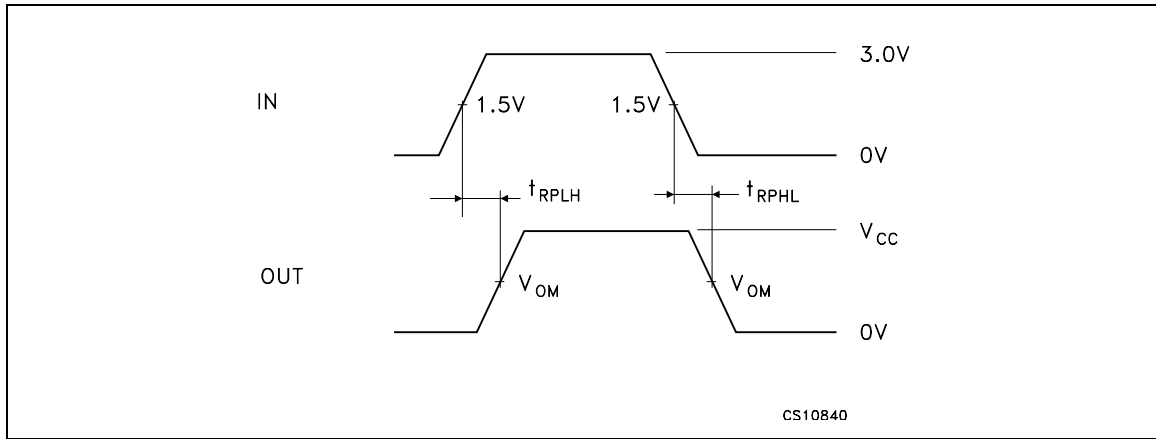
Figure 14. Receiver propagation delay time waveforms
