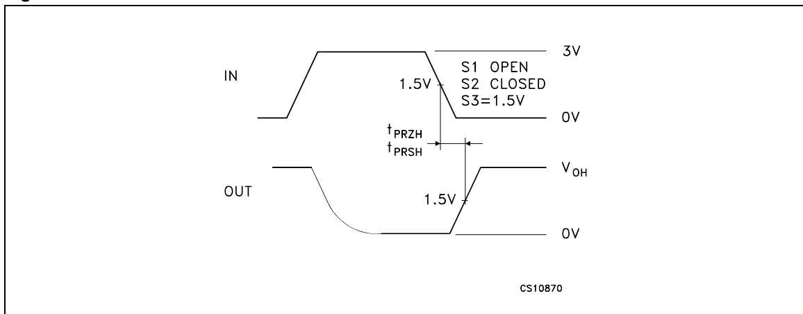
Figure 16. Receiver enable and disable times waveform
