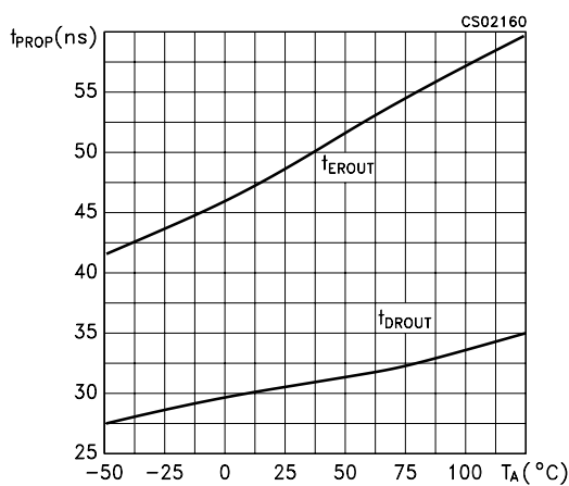
Figure 3 : Receiver Propagation Delay
