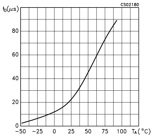
Figure 2 : INVALID LOW Threshold Time
