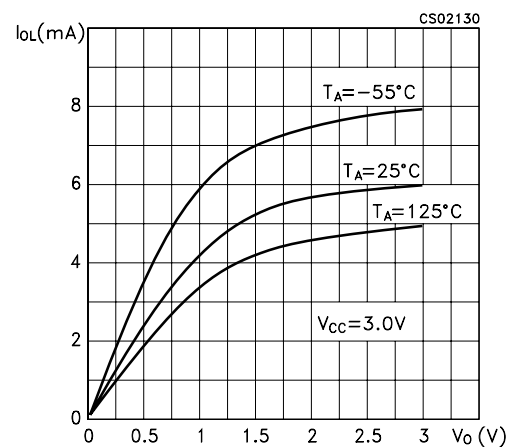
Figure 6 : Output Current vs Output Low Voltage
