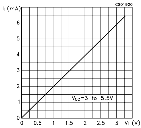
Figure 7 : Receiver Input Resistance
