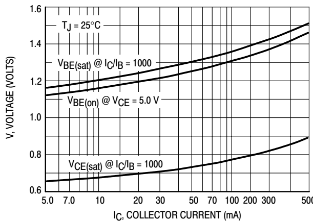
Figure 10. "On" Voltages
