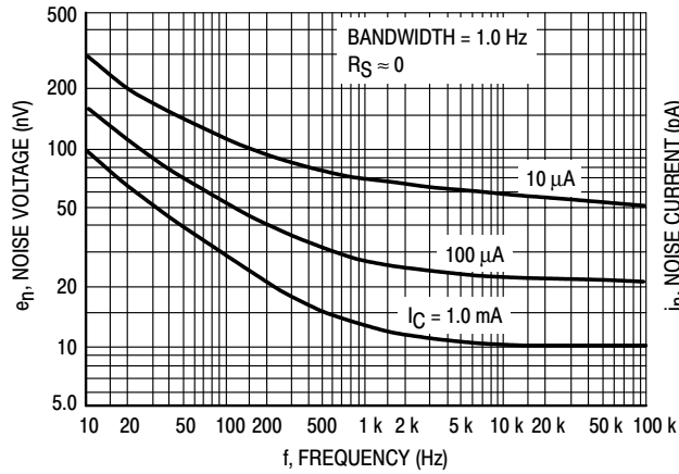
Figure 1. Noise Voltage
