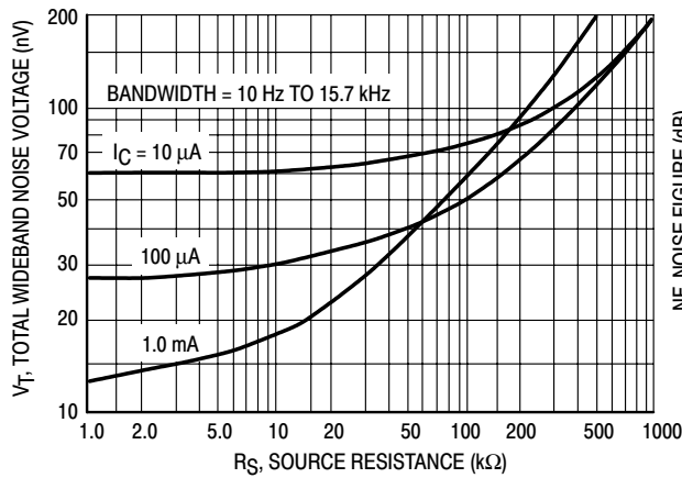
Figure 3. Total Wideband Noise Voltage
