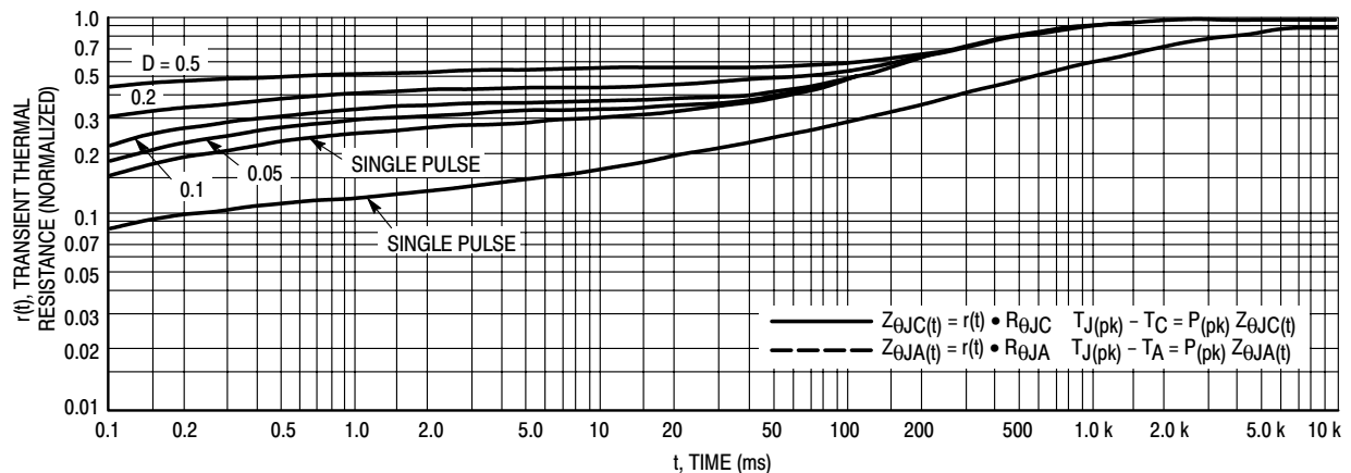
Figure 5. Thermal Response
