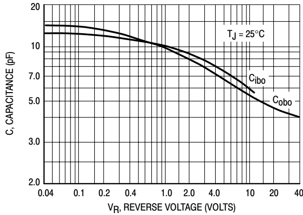
Figure 6. Capacitance
