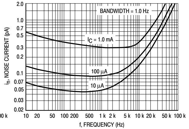
Figure 2. Noise Current
