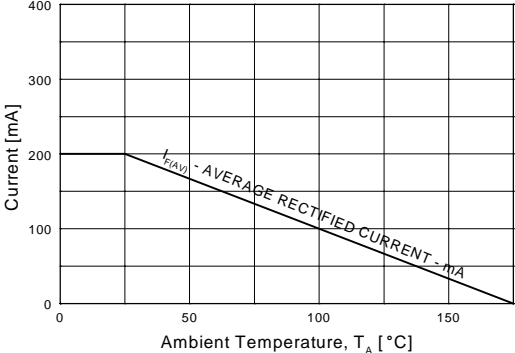
Figure 7. Average Rectified Current (I F(AV) ) versus Ambient Temperature (T A )
