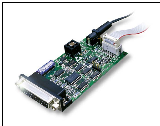
Figure 1: ST7-STICK Programmer
