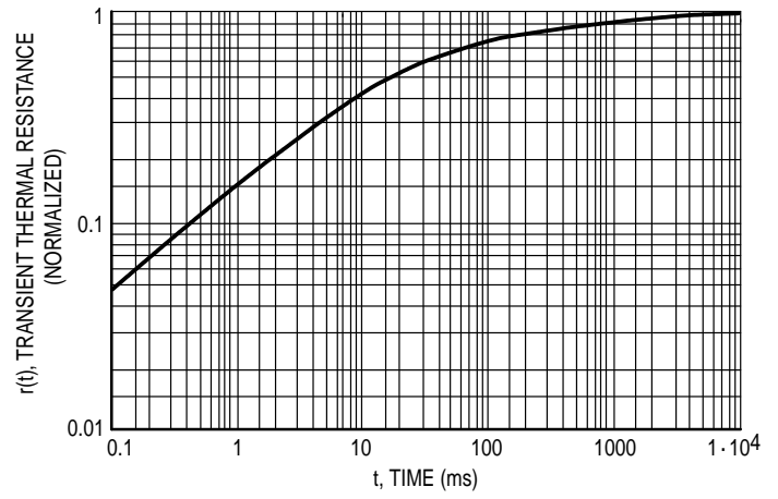
Figure 4. Thermal Response
