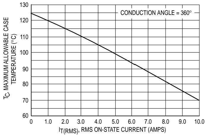
FIGURE 1 — CURRENT DERATING
