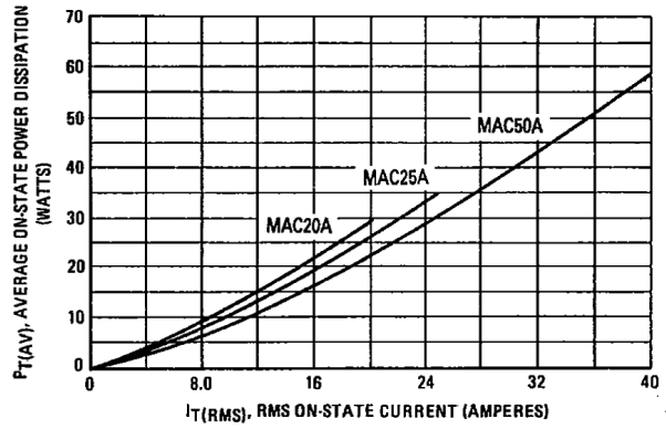
FIGURE 2 – MAXIMUM POWER DISSIPATION
