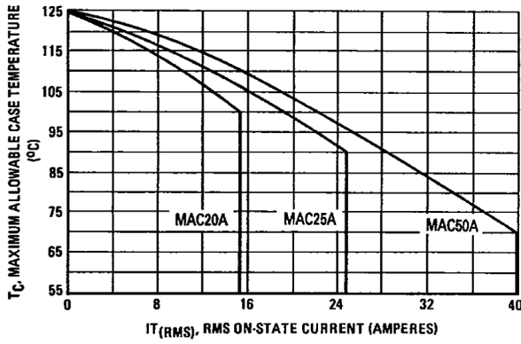
FIGURE 1 – CURRENT DERATING
