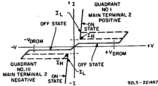
Fig. 1 - Principal voltage-current characteristic.
