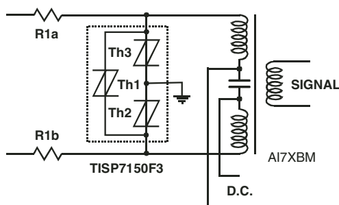
Figure 22. ISDN Protection
