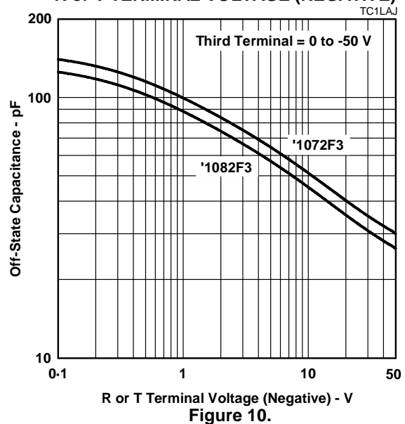
OFF-STATE CAPACITANCE VS R or T TERMINAL VOLTAGE (NEGATIVE)
