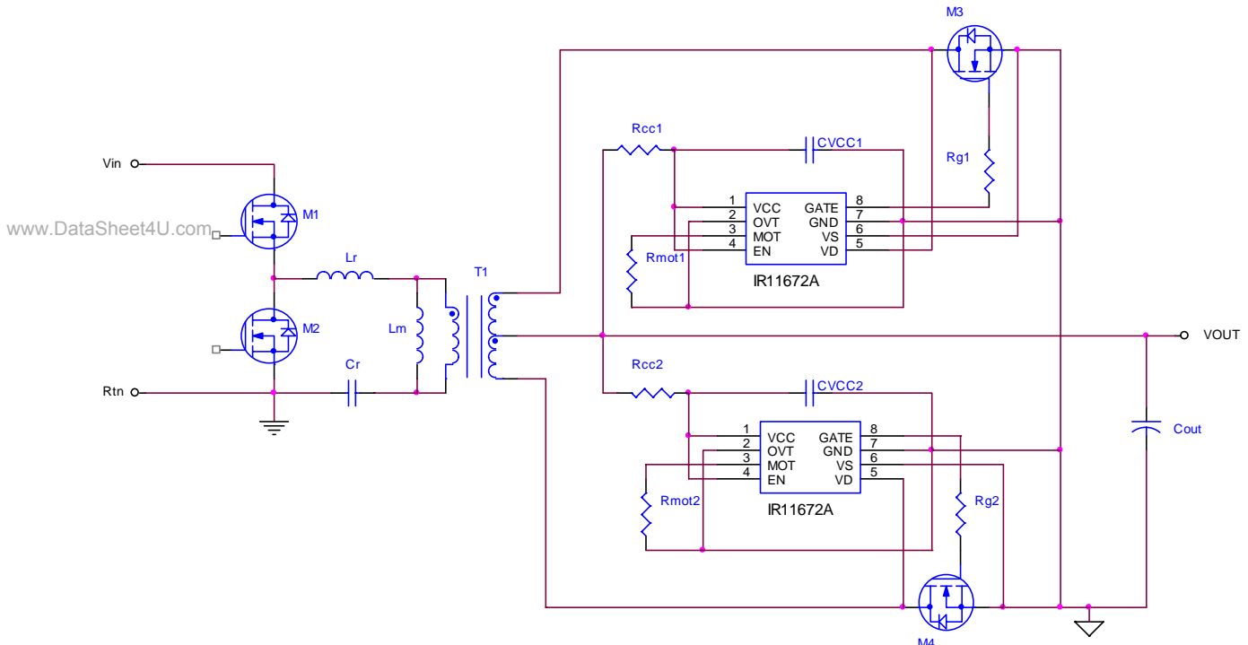
Figure 7: Resonant half-bridge application circuit
