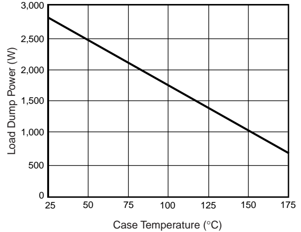
Load Dump Power Characteristics (10ms Exponential Waveform)
