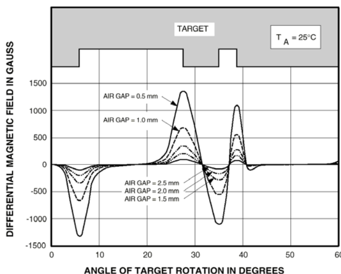
Figure 4. Affect of varying air gaps on differential sensors.
