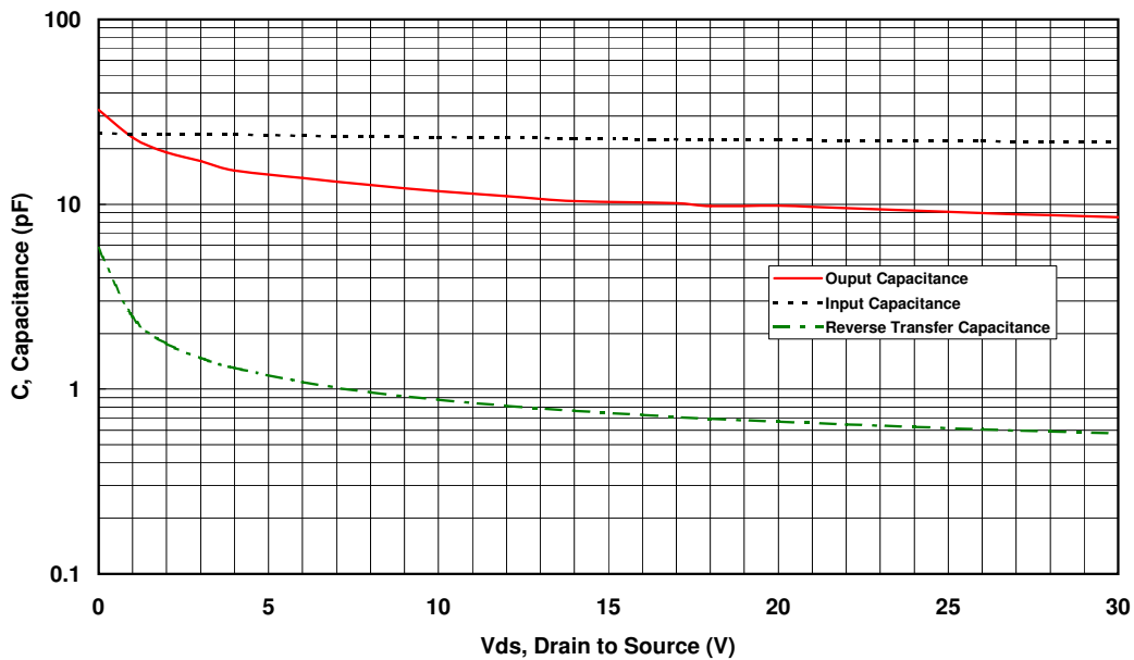
Figure 6 – Typical CV Characteristics.
