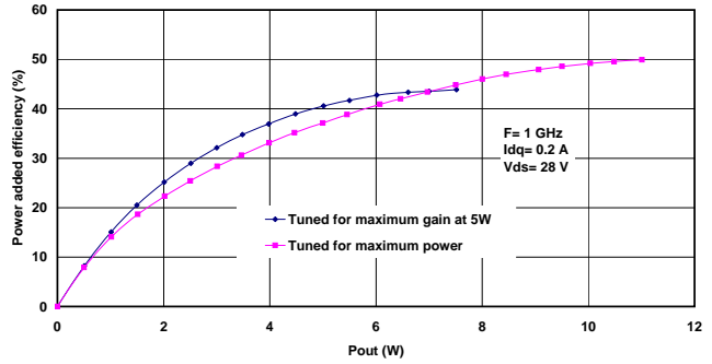
Figure 2 Power added efficiency vs. Output Power
