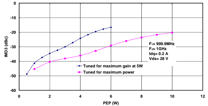
Figure 4 IMD 3 vs. PEP
