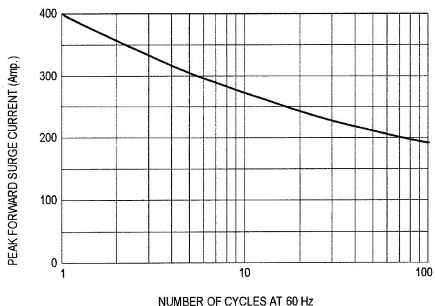
NUMBER OF CYCLES AT 60 Hz
