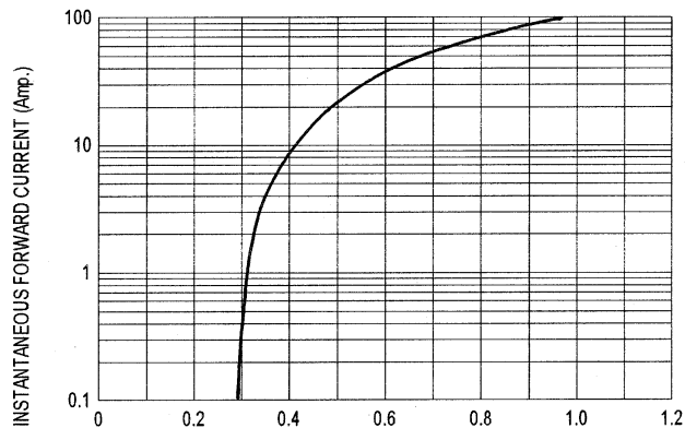
FIG-2 TYPICAL FORWARD CHARACTERISTICS
