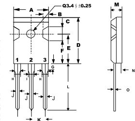
TO-247 (3P)
