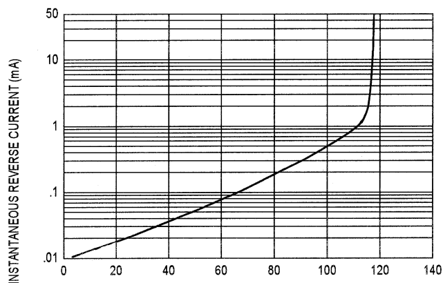
PERCENT OF PEAK REVERSE VOLTAGE(%)
