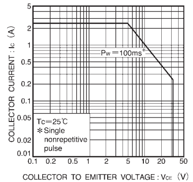
Fig.9 Safe operating area (2SD1758)
